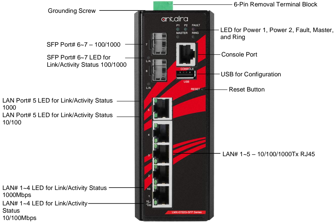
Figure 2.2 - The Front Panel of LMX-0702G-SFP-V2 Series
